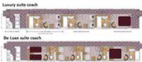
Wagon Layout
